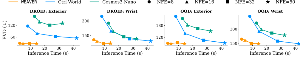
Figure 2: We present FVD vs inference time (seconds) across views on DROID and OOD datasets, where WEAVER pareto-dominates baselines for different NFEs while using 16 \times less inference time.
