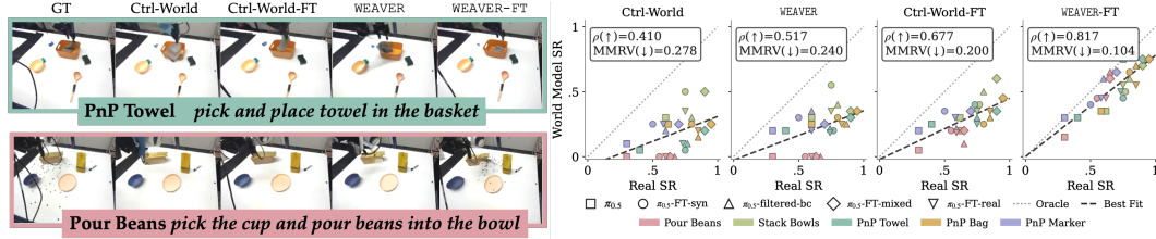
Figure 5: (Left) For PnP Towel, only WEAVER and WEAVER-FT accurately imagine the towel inside the basket. For Pour Beans, only WEAVER-FT captures the beans scattering across the table. (Right) Evaluation inside WEAVER-FT attains high rank correlation with real-world success rates.
