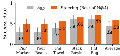
Figure 7: We show test-time steering with WEAPER outperforms the \pi_{0.5} by 14%.
