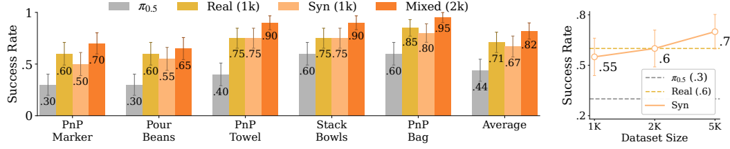
Figure 6: (Left) We finetune \pi_{0.5} with multiple data sources and combining real and synthetic (Syn) obtained with WEAPER outperforms other variants. (Right) We ablate the number of segments in synthetic data for finetuning and report the success rate across 20 trials for the Pour Beans Task.
