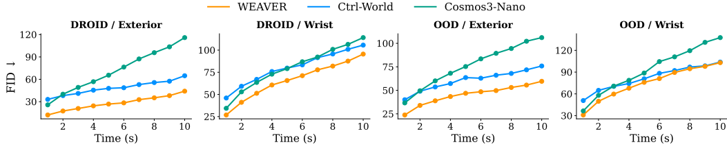
Figure 3: We report FID at various horizon lengths (in seconds) and observe that WEAVER is consistently better at long-horizon rollouts compared to Ctrl-World and Cosmos3-Nano.
