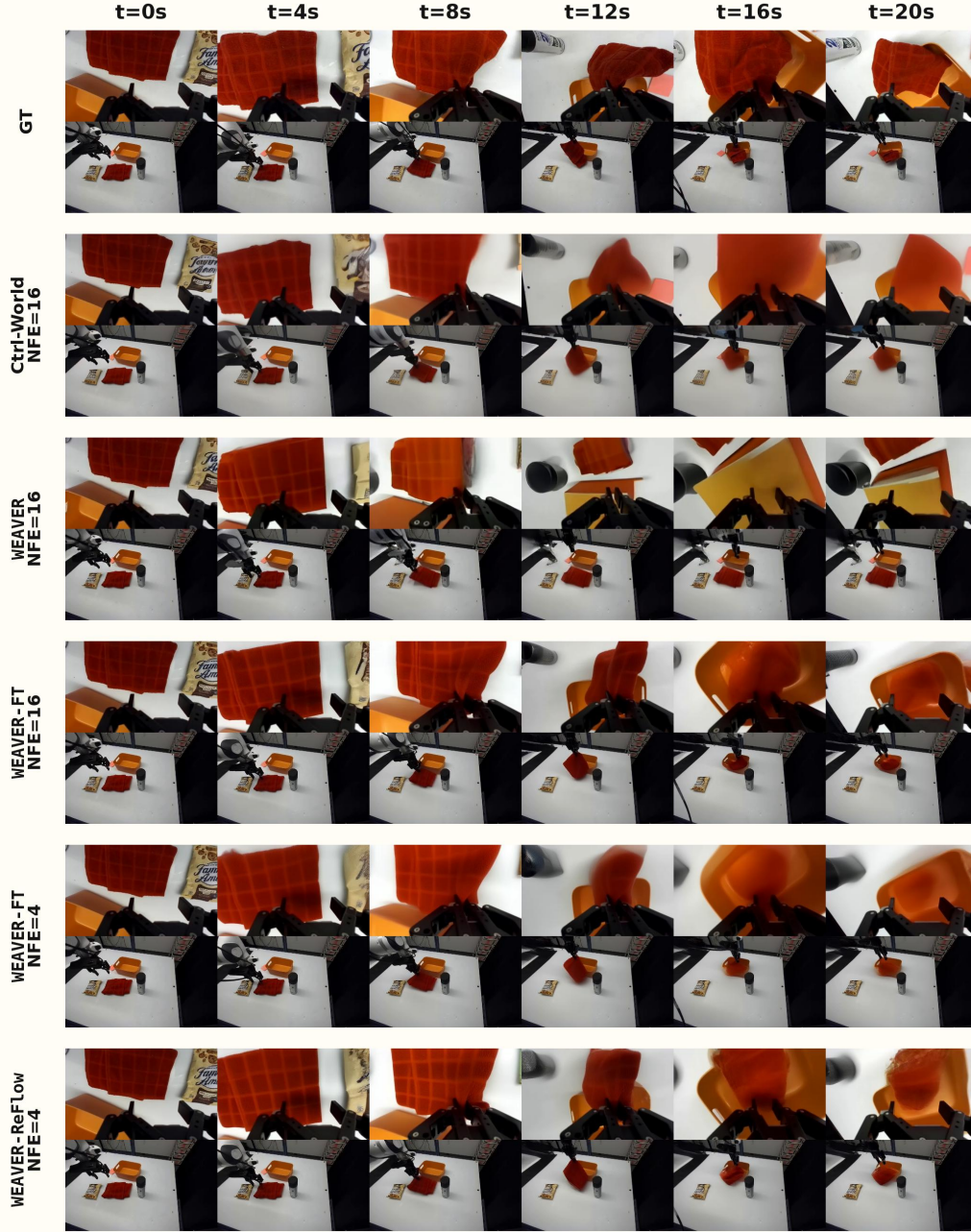
Figure 15: We compare the rollouts on task obtained from Ctrl-World, WEAVR, WEAVR-FT and WEAVR-REFLOW at different NFE values of 4 and 16. We generate rollouts for 20 seconds and present predicted camera views at every 4 second. We observe that WEAVR-REFLOW is better than WEAVR-FT at NFE=4 and is more consistent than Ctrl-World and WEAVR with NFE=16.
