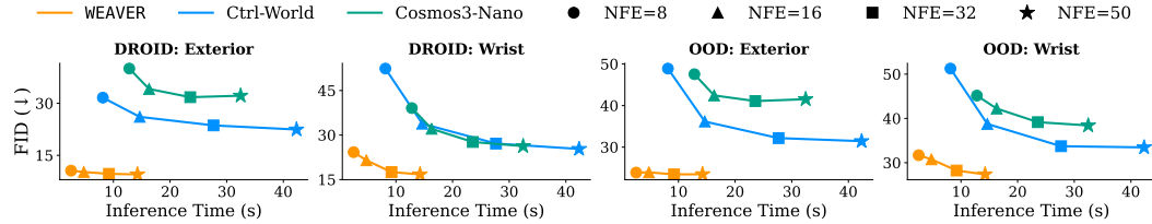
Figure 10: We compare FID vs inference time for WEAVER and Ctrl-World and find that WEAVER outperforms the baseline even when the baseline uses up to 16x more inference time
